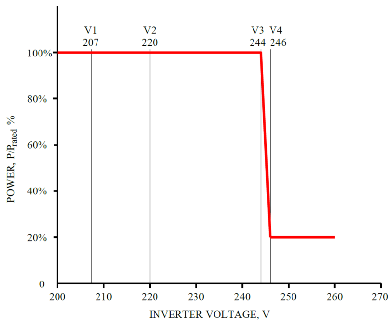
Figure 4 Required Volt-Watt response mode
